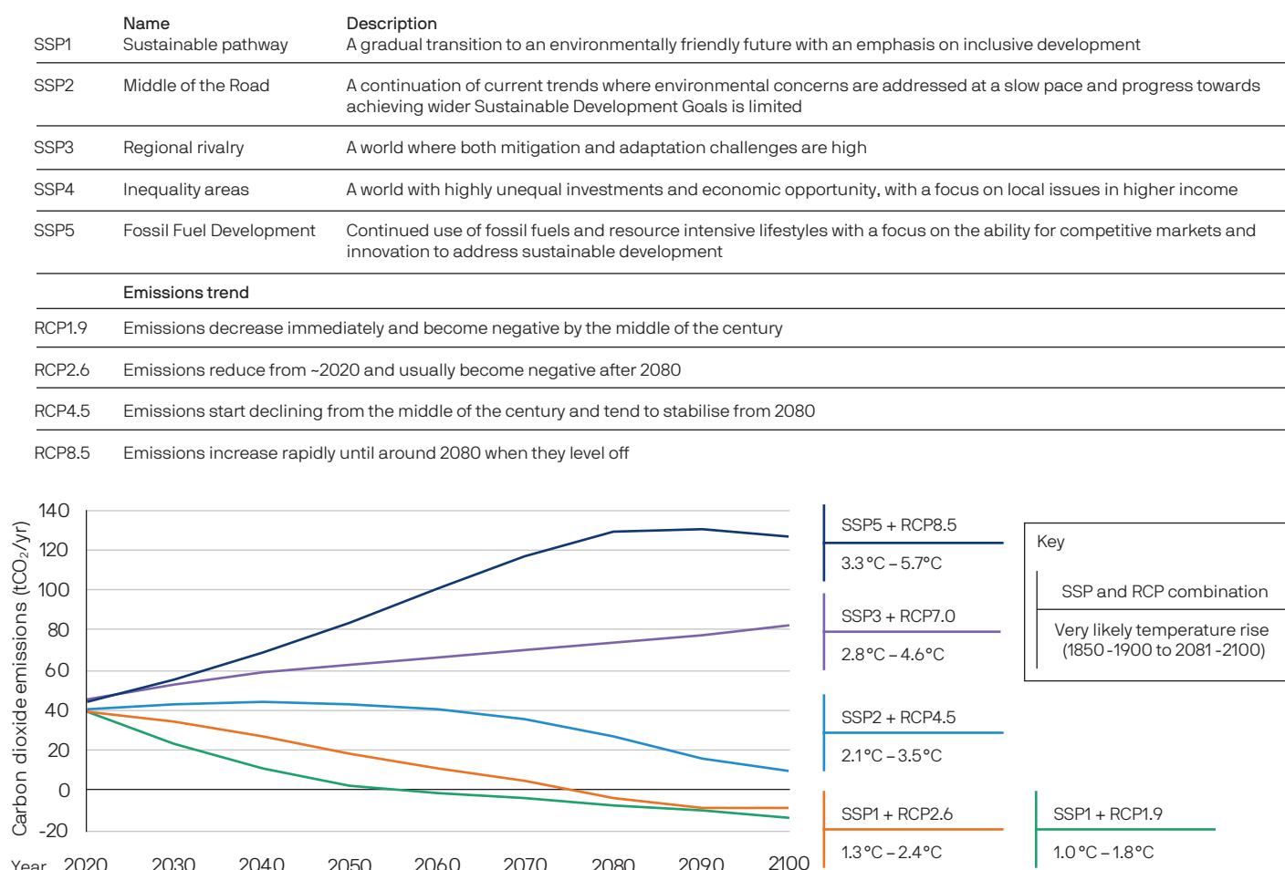
Exhibit 3: Summary of SSP storylines, RCP emissions trends and temperature outcomes 6, 7, 8, 9
